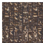
F3665001 Diorite
